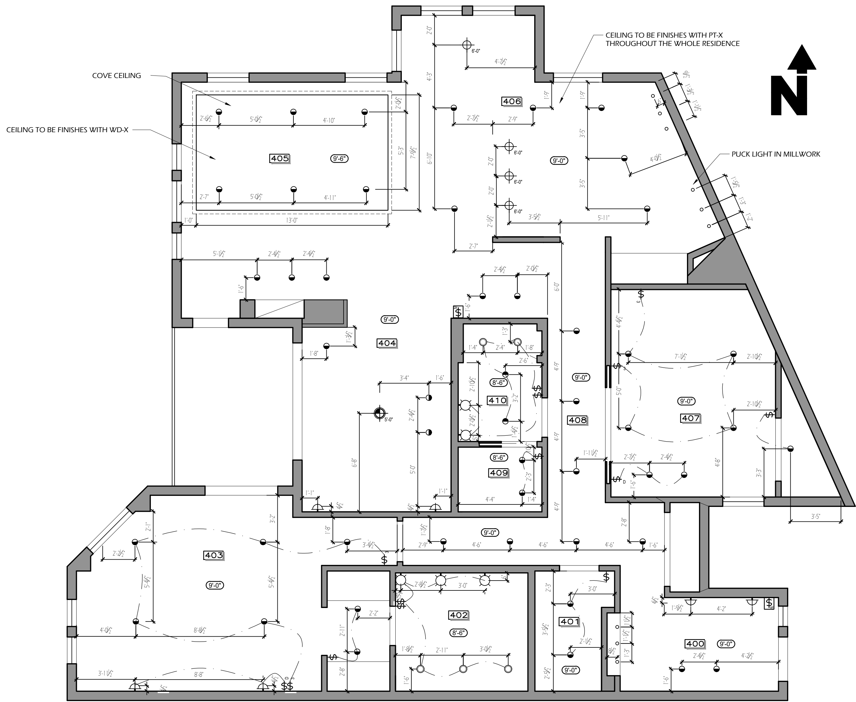
1 REFLECTED CEILING PLAN SCALE: 1/4" = 1'-0"
