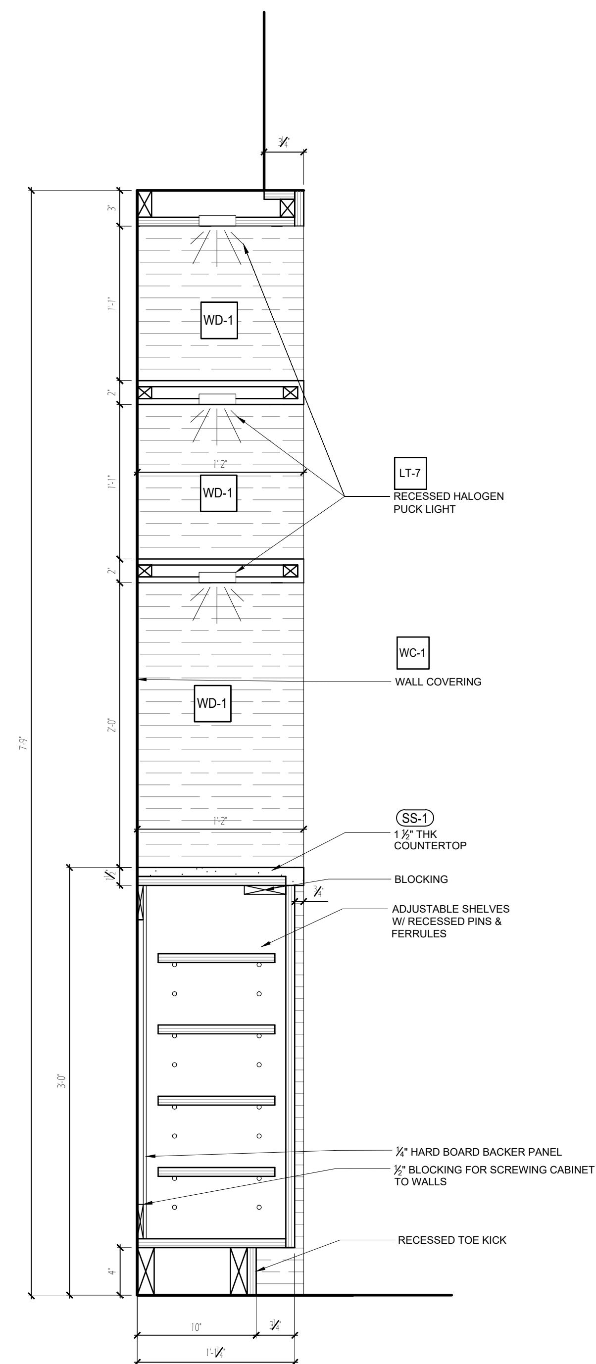
1 SECTION - ENTRY CABINETS ID.1.07 SCALE: 1 1/2" = 1'-0"
