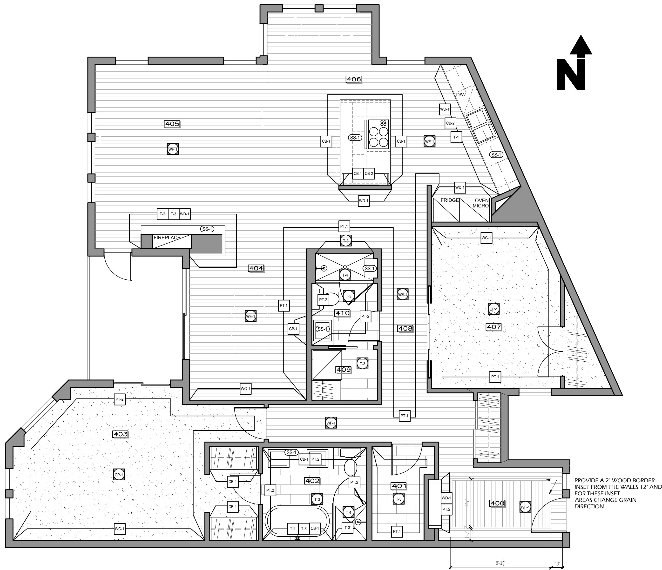
1 FINISHES PLAN ID1.05 SCALE: 1/4" = 1'-0"
