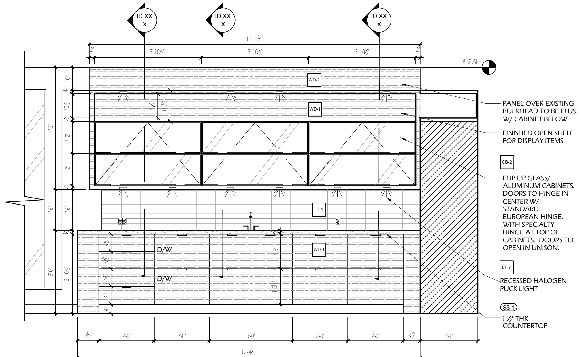
2 ELEVATION - KITCHEN (SINK WALL) SCALE: 1/2" = 1'-0"
