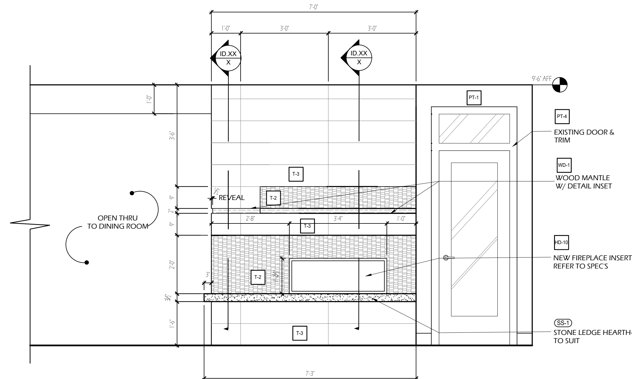
5 ELEVATION - FIREPLACE + FLOATING HEARTH SCALE: 1/2" = 1'-0"
