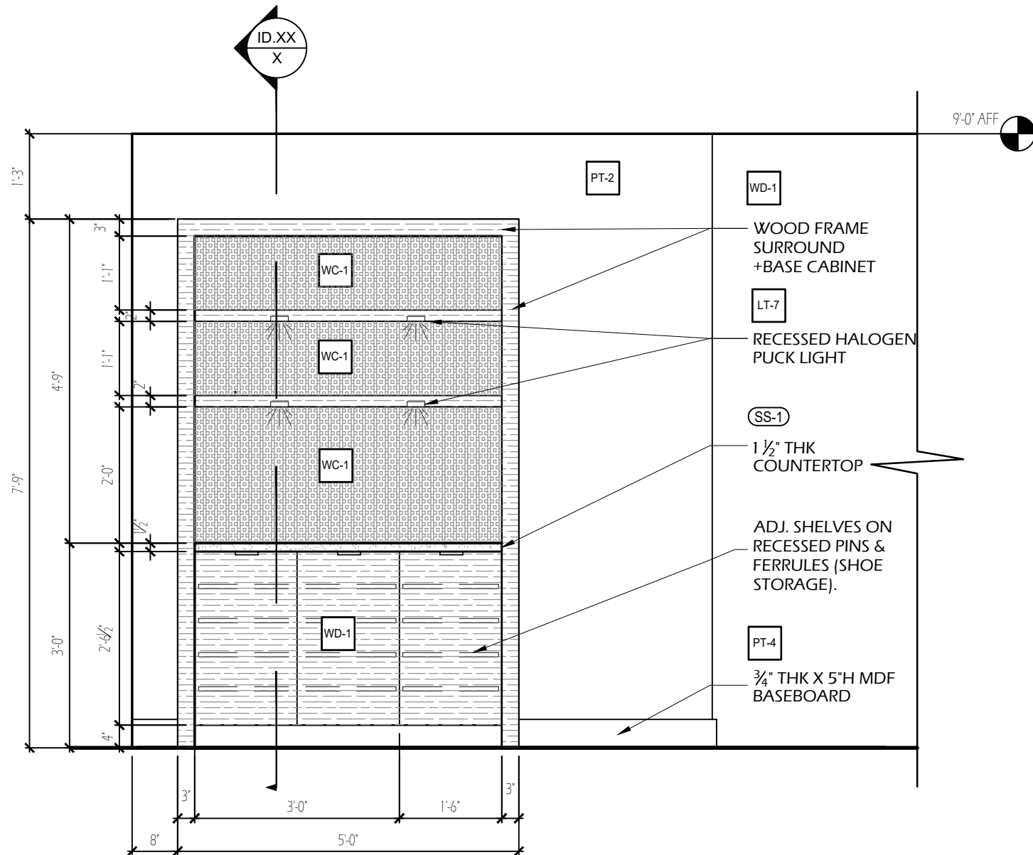
1 ELEVATION - ENTRY (SHOE CLOSET) SCALE: 1/2" = 1'-0"
