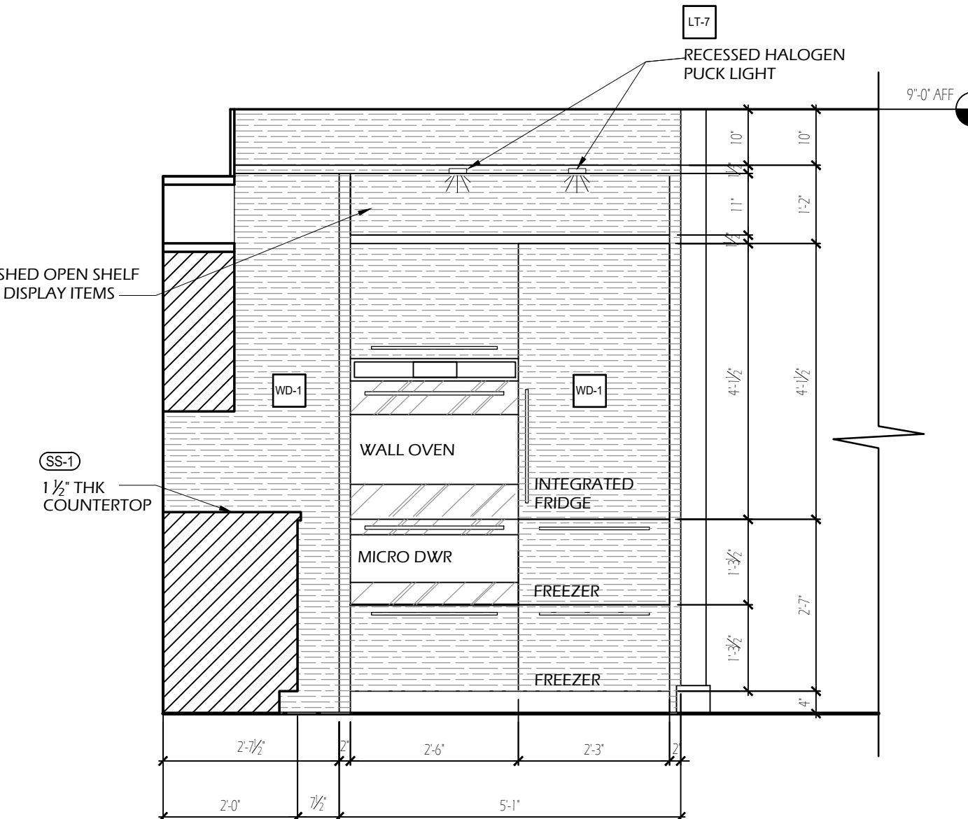
3 ELEVATION - KITCHEN (FRIDGE WALL/ OVEN) SCALE: 1/2" = 1'-0"
