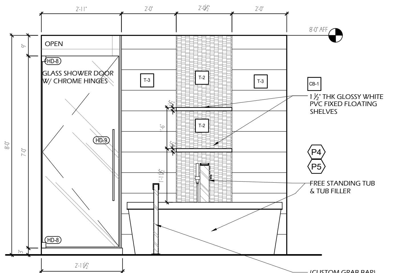
4 ELEVATION - PRIMARY ENSUITE (SHOWER/ TUB WALL) SCALE: 1/2" = 1'-0"
