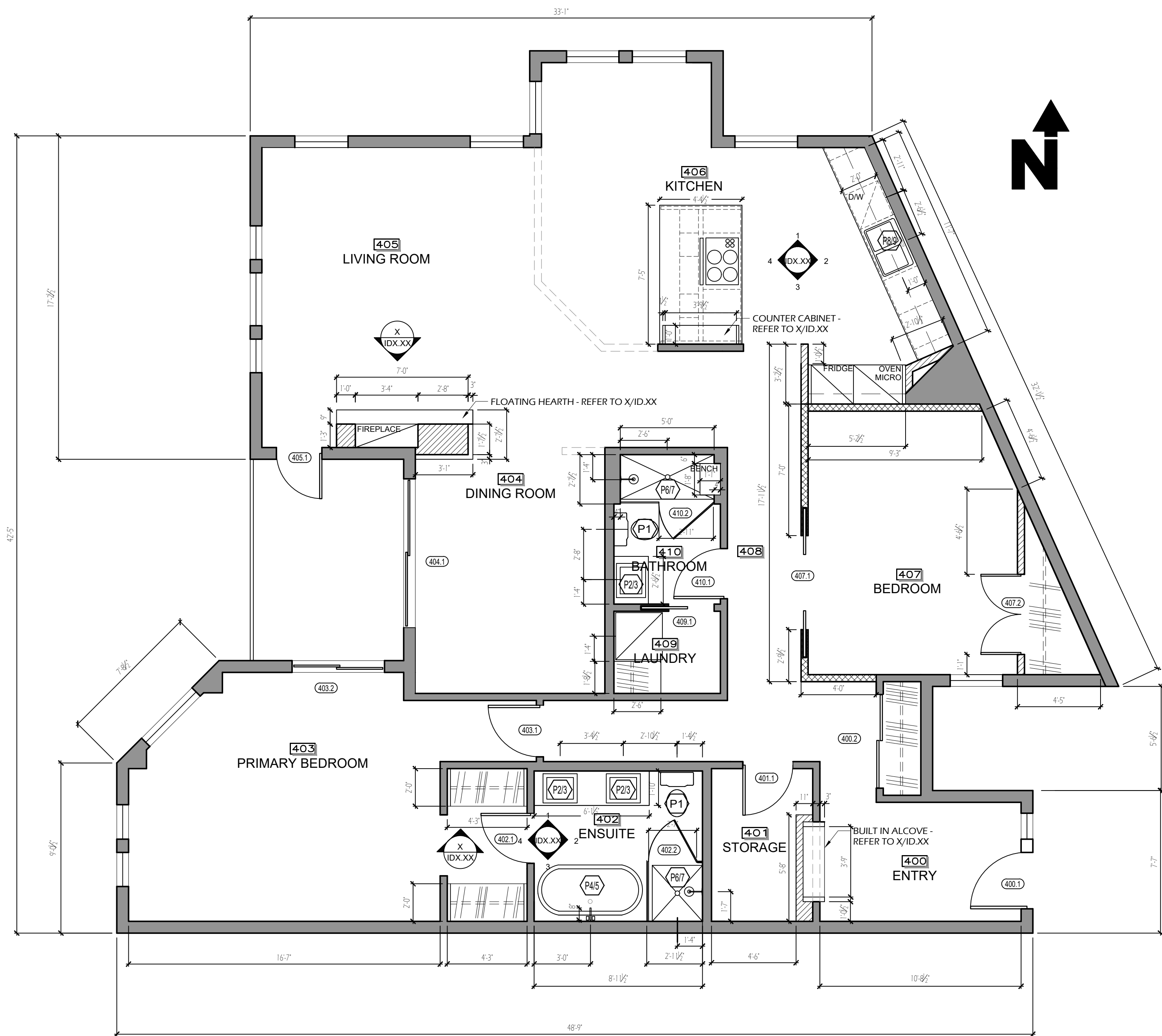
1 PRESENTATION PLAN SCALE: 1/4" = 1'-0"
