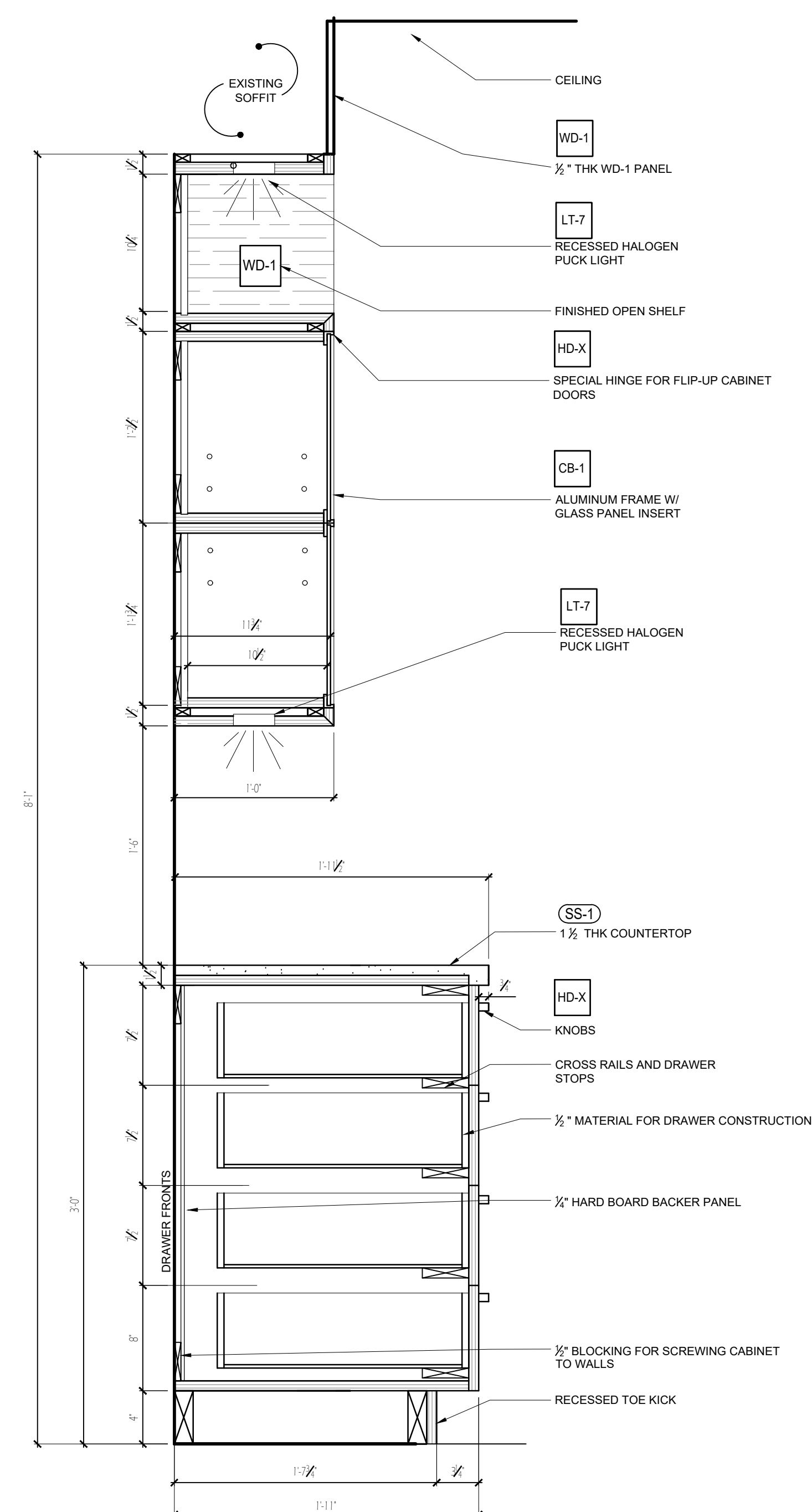
2 SECTION - KITCHEN CABINETS ID.1.07 SCALE: 1 1/2" = 1'-0"
